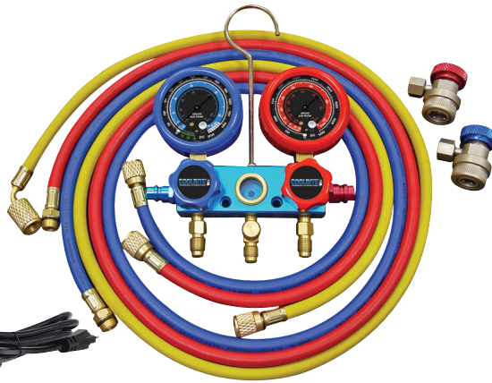
MC 289772-CL R134a Aluminum Manifold Gauge Set
